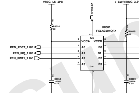
LEVEL SHIFTER
