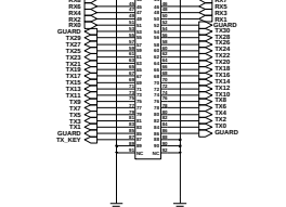
90Pin TSP Connector
