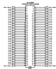
70pin S-PEN Connector
