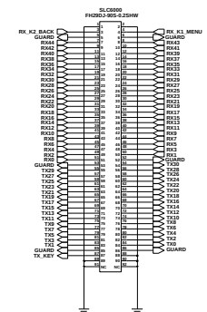
90Pin TSP Connector
