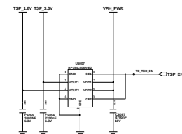
TSP Dual LDO
