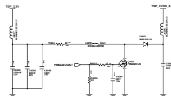
XVDD Booster Discrete
